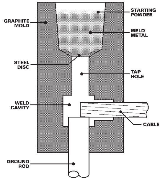
Cutaway Section of CR-1 Type Mold
